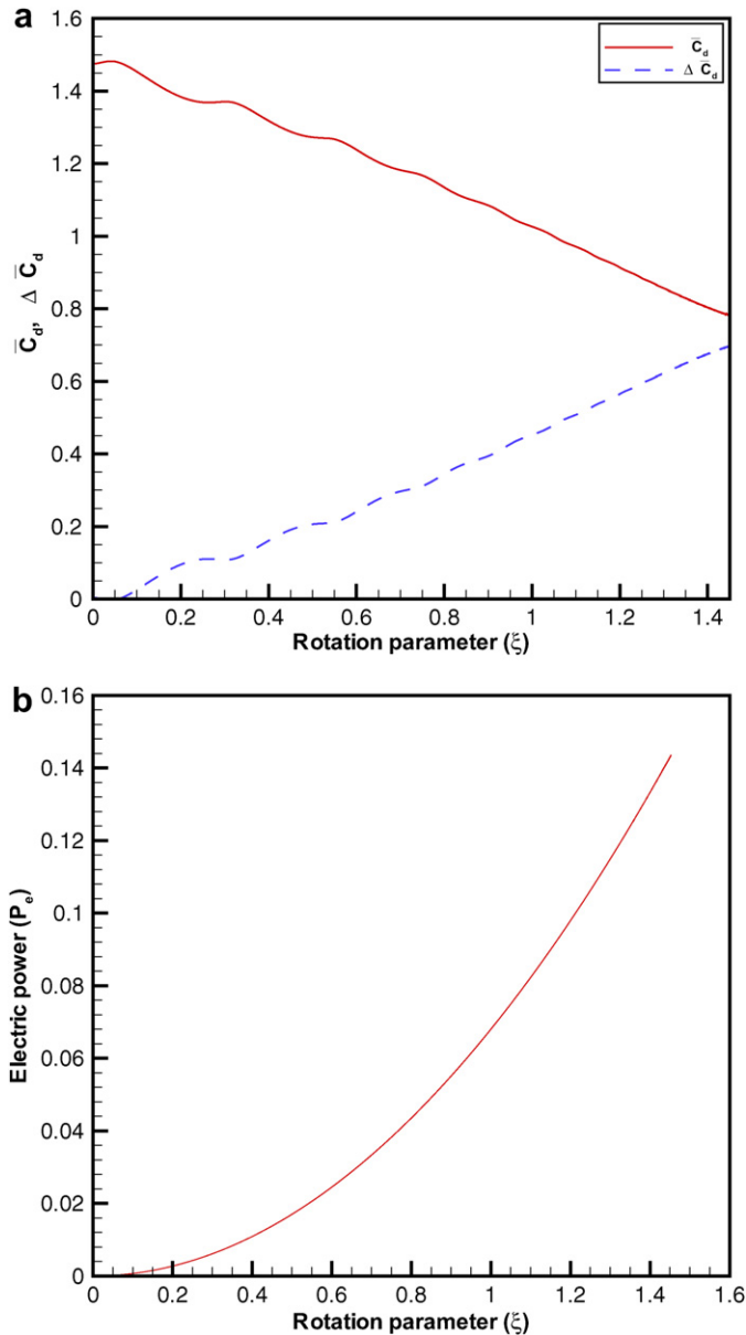
Fig. 17. (a) Variation of mean drag coefficient ( \bar{C}_d ) and net drag savings ( \Delta \bar{C}_d = \bar{C}_{d_{iso}} - \bar{C}_{d_i} ) with rotation parameter and (b) Modeled electric power consumption with rotation parameter for Re = 100 .
