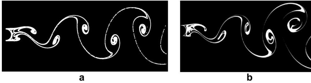
Fig. 4. Validation for (a) numerically resolved streaklines for Re = 100 (b) experimental visual of Taneda [38] for Re = 140 . Note in particular, the remarkable similarity in the eddy shedding process and the connection between all the shed eddies through an umbilical chord .
