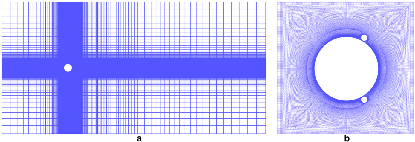
Fig. 3. (a). Discretization of the computational domain and (b), a close-up view of the grid resolution in the vicinity of the main cylinder.
